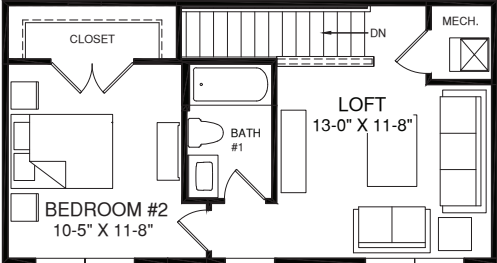
UPPER LEVEL
