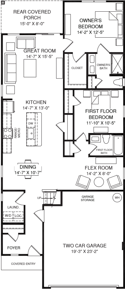
MAIN LEVEL
