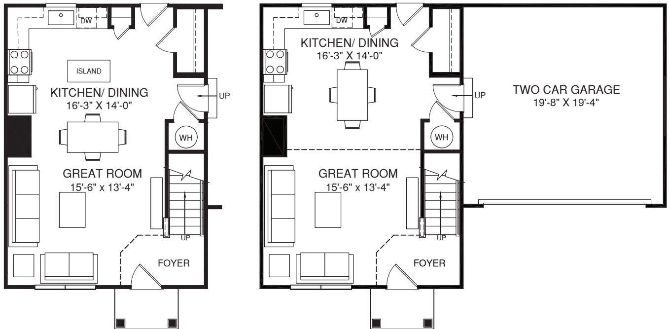
MAIN LEVEL
