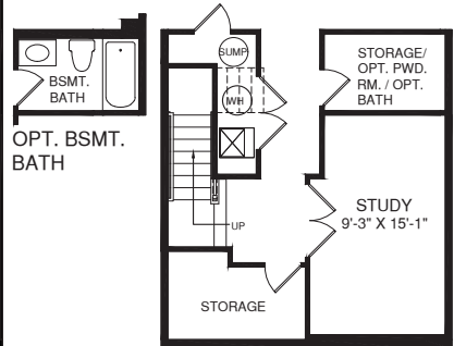
OPT. STUDY
