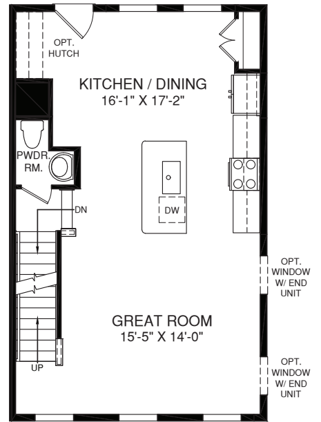
MAIN LEVEL
