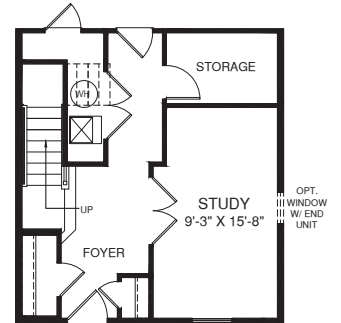
LOWER LEVEL
