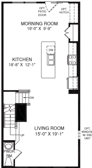
MAIN LEVEL
