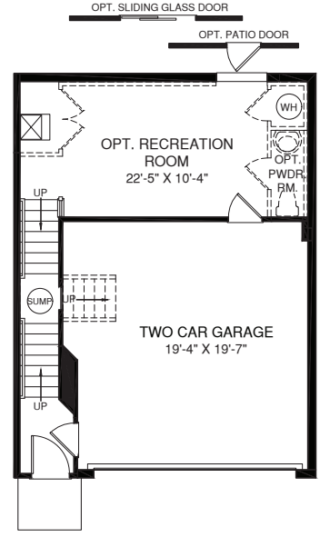
LOWER LEVEL
