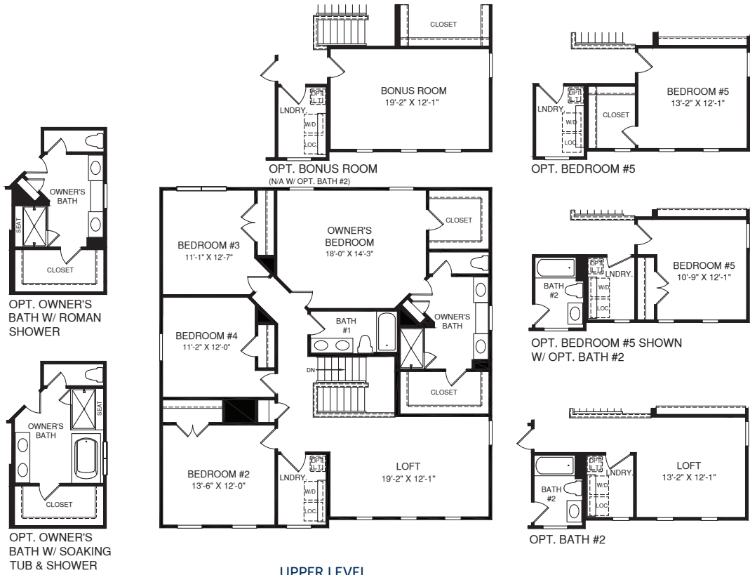
UPPER LEVEL
