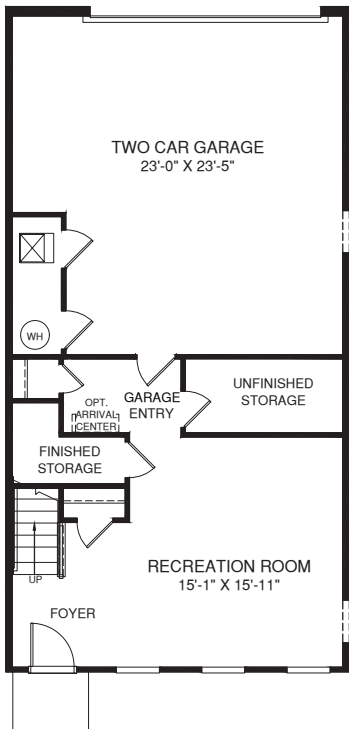
LOWER LEVEL
