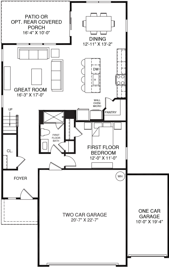
MAIN LEVEL
