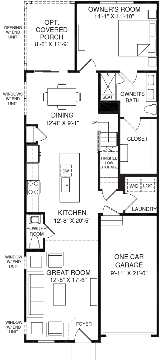
MAIN LEVEL
