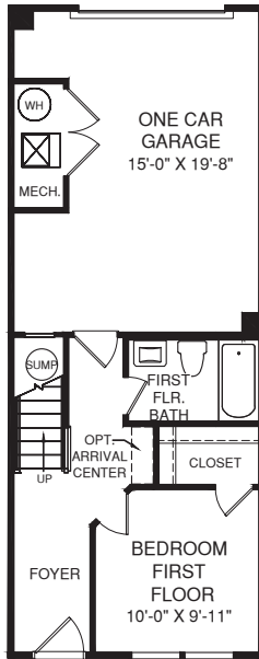
ONE CAR GARAGE SHOWN W/ OPT. BEDROOM
