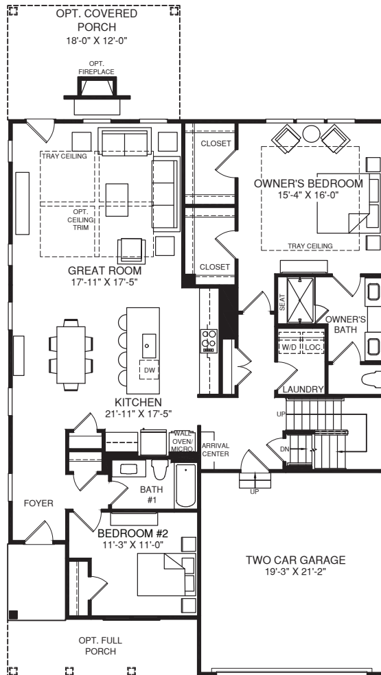
MAIN LEVEL
