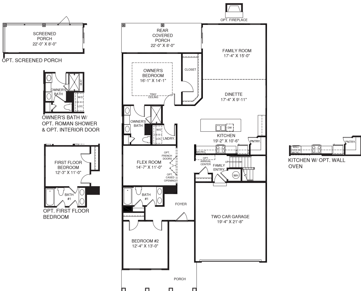
MAIN LEVEL
