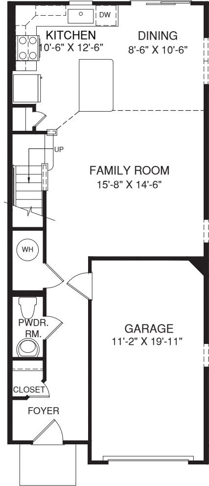
MAIN LEVEL
