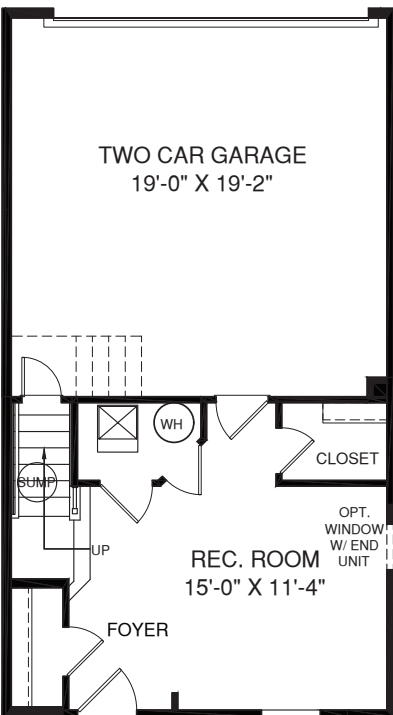
LOWER LEVEL
