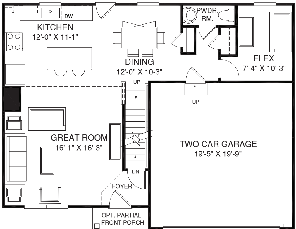
MAIN LEVEL
