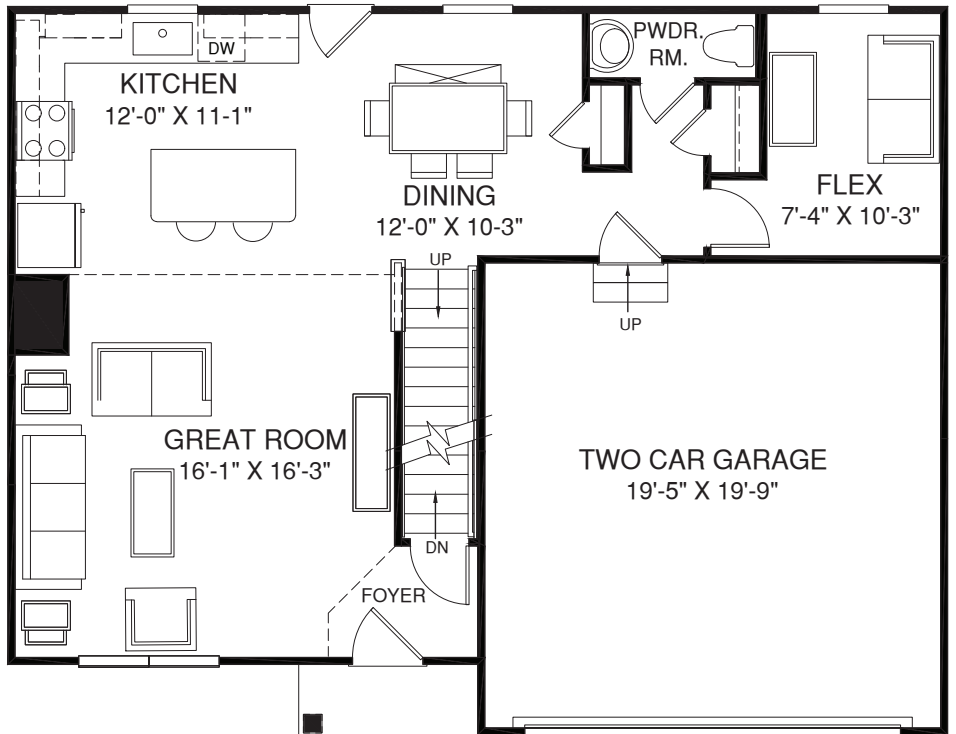
MAIN LEVEL
