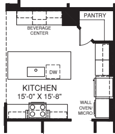
OPT. KITCHEN LAYOUT
