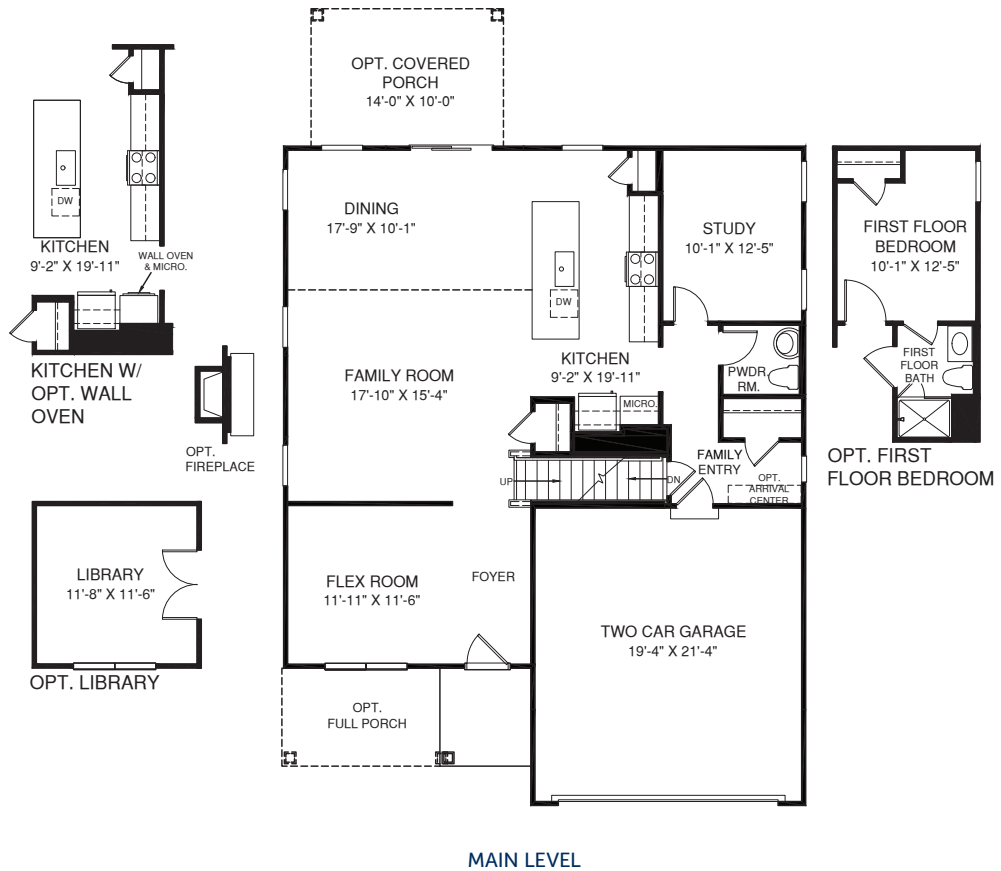
MAIN LEVEL
