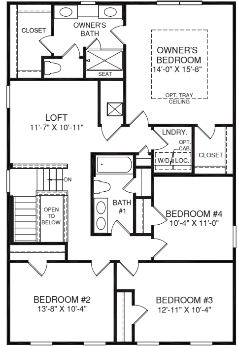
UPPER LEVEL
