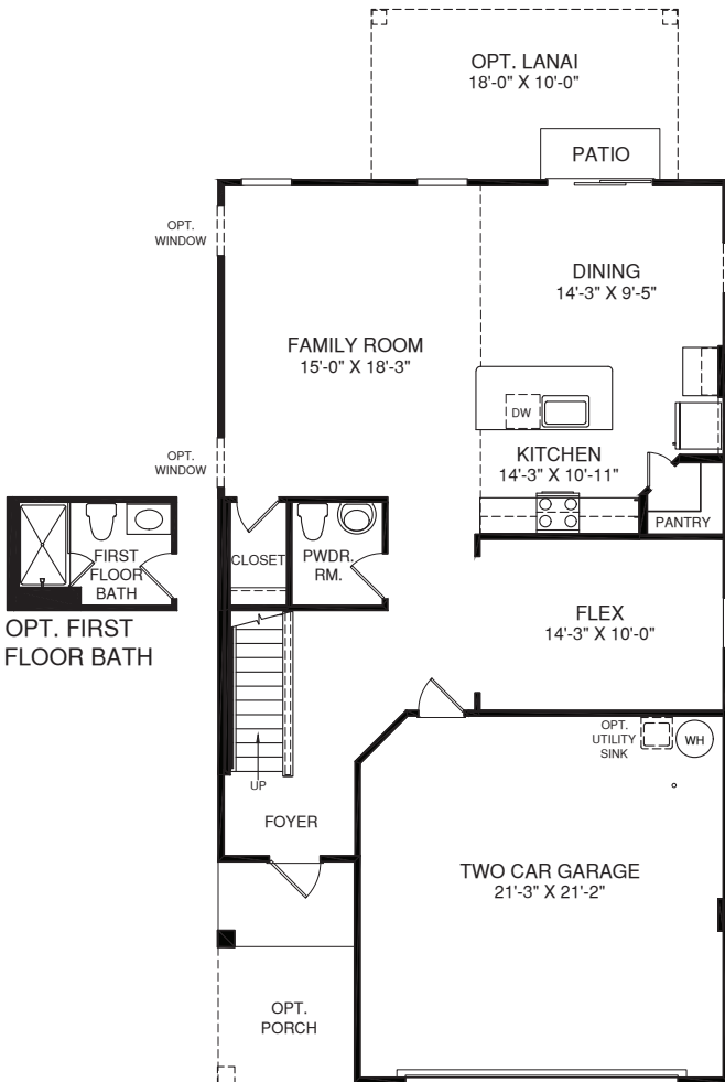
MAIN LEVEL
