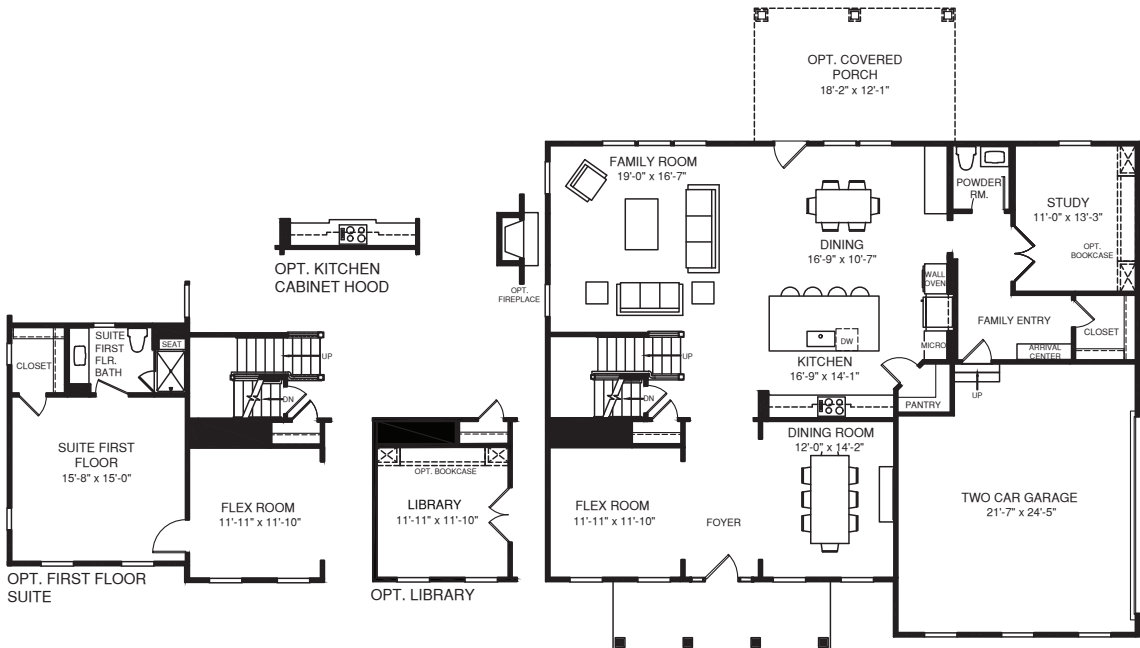
MAIN LEVEL
