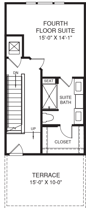
OPTIONAL SUITE FOURTH FLOOR
