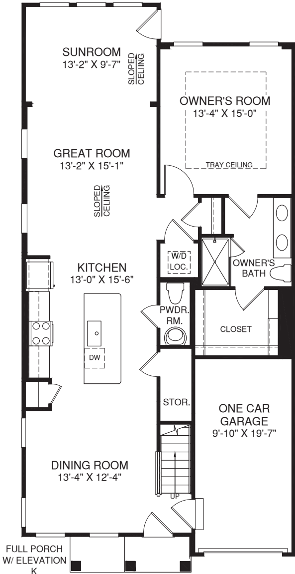
MAIN LEVEL
