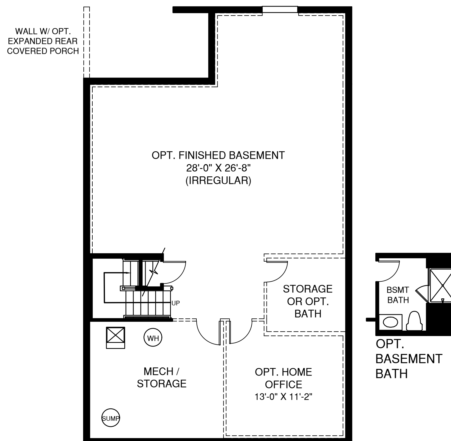
LOWER LEVEL
