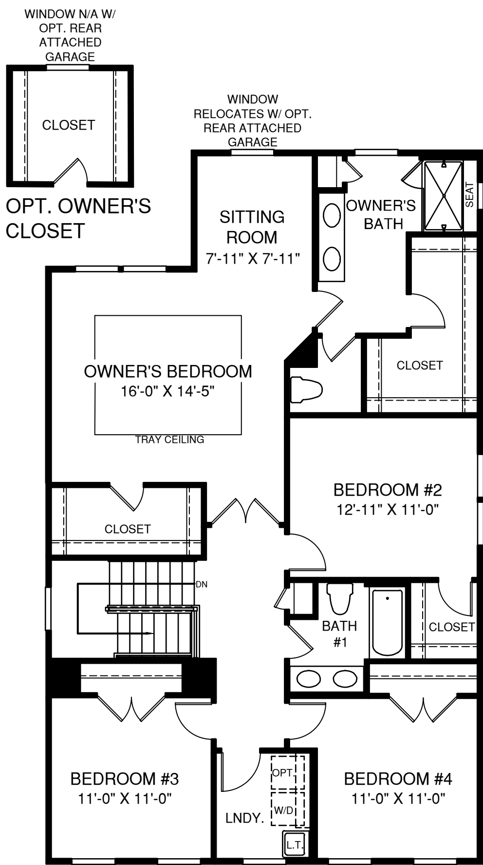
UPPER LEVEL
