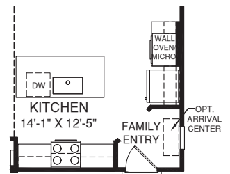
KITCHEN W/ OPT. WALL OVEN
