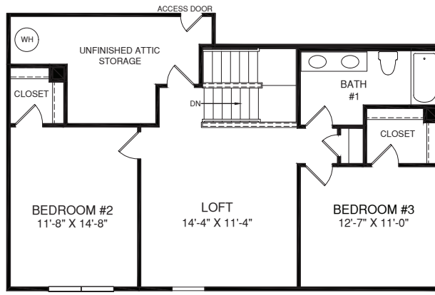
UPPER LEVEL
