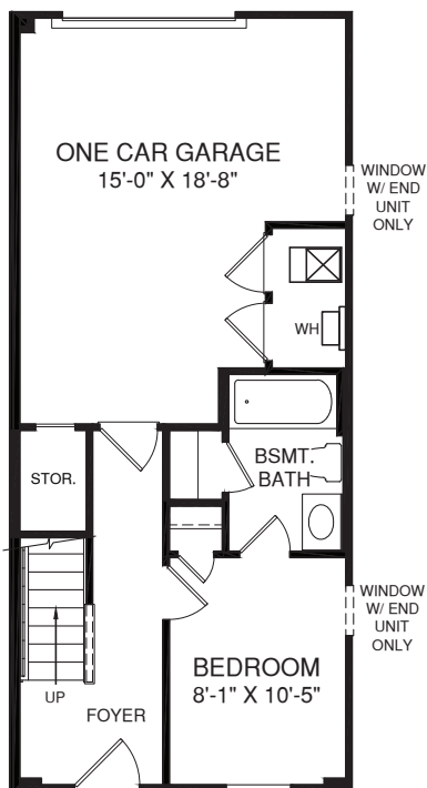
LOWER LEVEL
