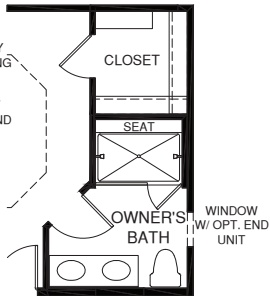
OPT. OWNER'S BATH SHOWER ALT. LAYOUT
