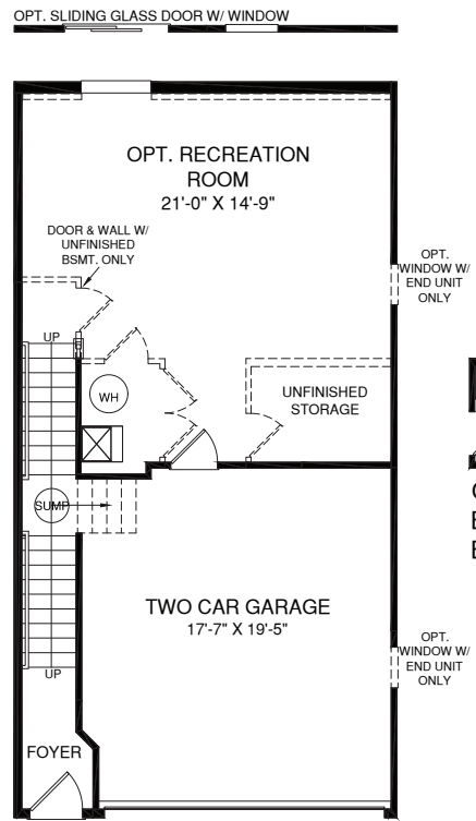
LOWER LEVEL
