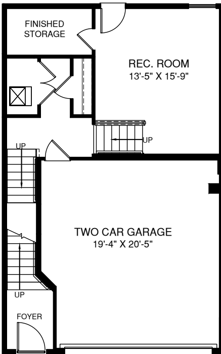
STEP DOWN BASEMENT LAYOUT
