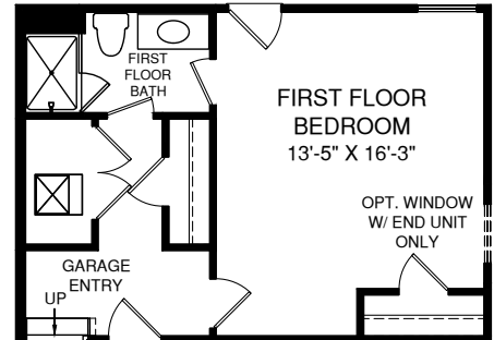
OPT. FIRST FLOOR BEDROOM SHOWN W/ OPT. BSMT BATH
