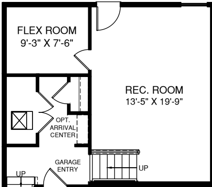
OPT. 4'-0" EXTENSION TO HOUSE
