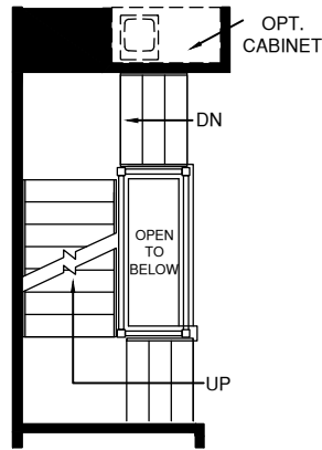
STAIRS TO OPT. FOURTH FLOOR
