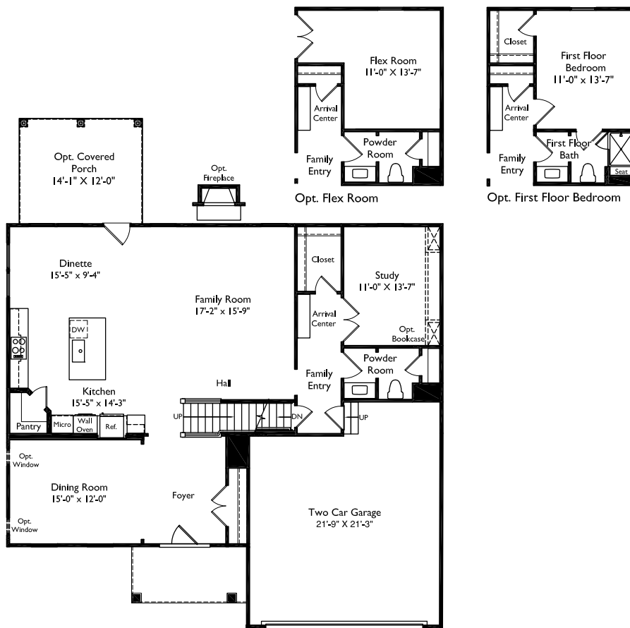
MAIN LEVEL
