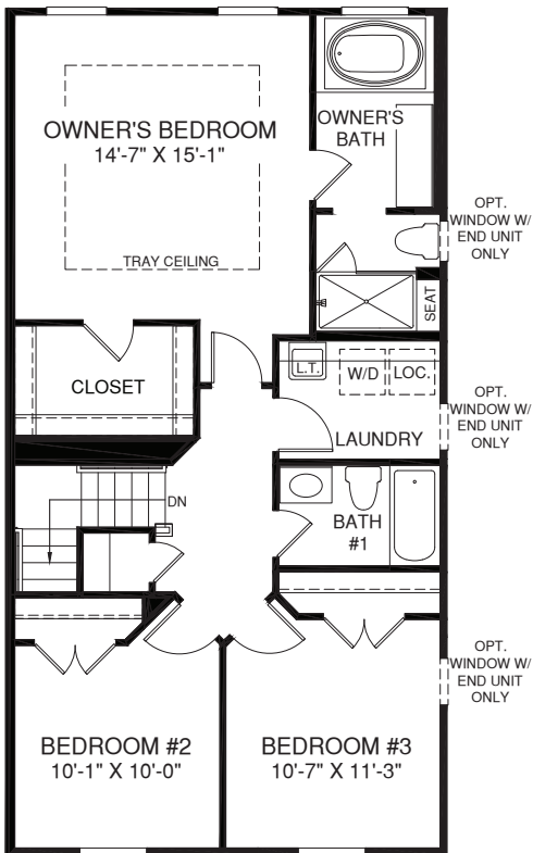
UPPER LEVEL
