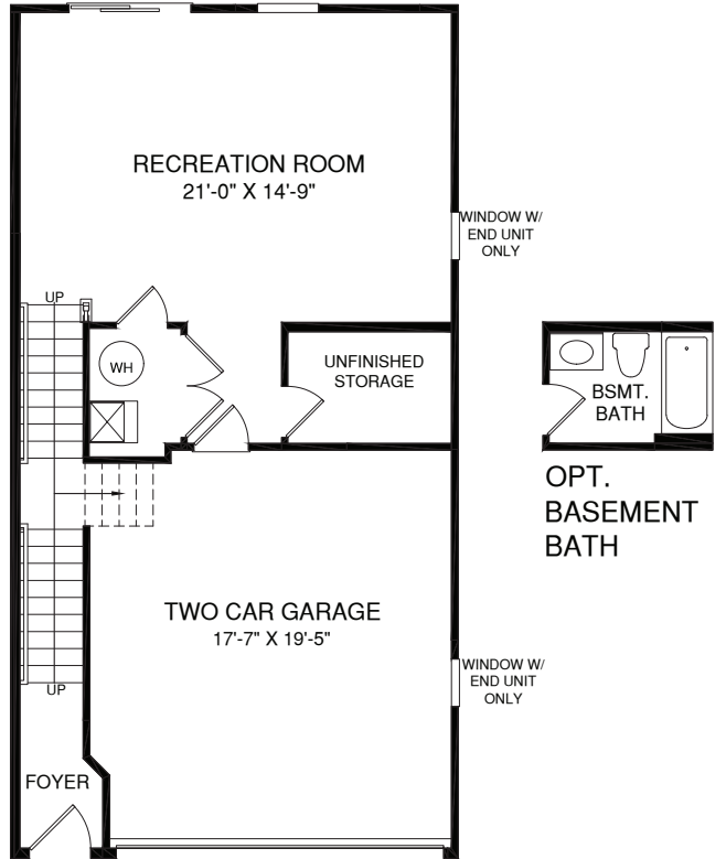
LOWER LEVEL
