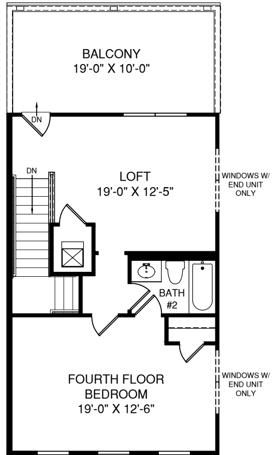
FOURTH FLOOR PLAN W/ ELEVATIONS #1 AND #3
