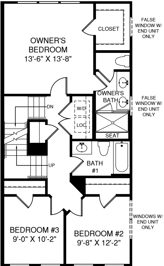
OPT. 3RD BEDROOM LAYOUT
