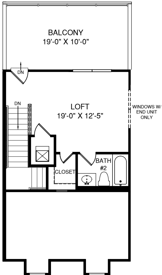
FOURTH FLOOR PLAN W/ ELEVATIONS #2,#4 AND #5
