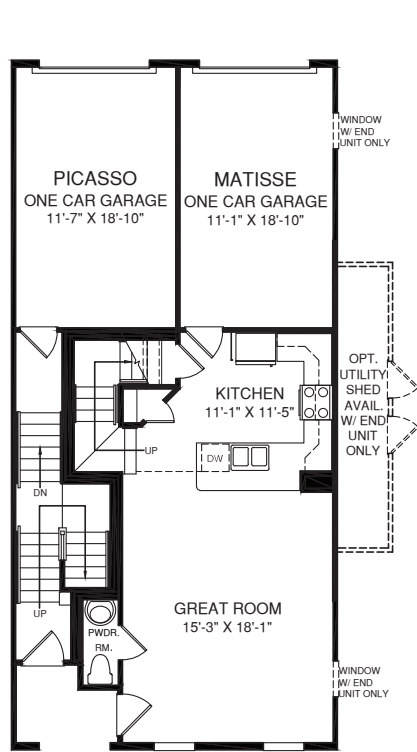
FIRST FLOOR MATISSE MAIN LEVEL
