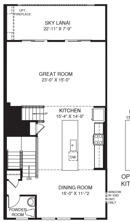
THIRD FLOOR PICASSO MAIN LEVEL
