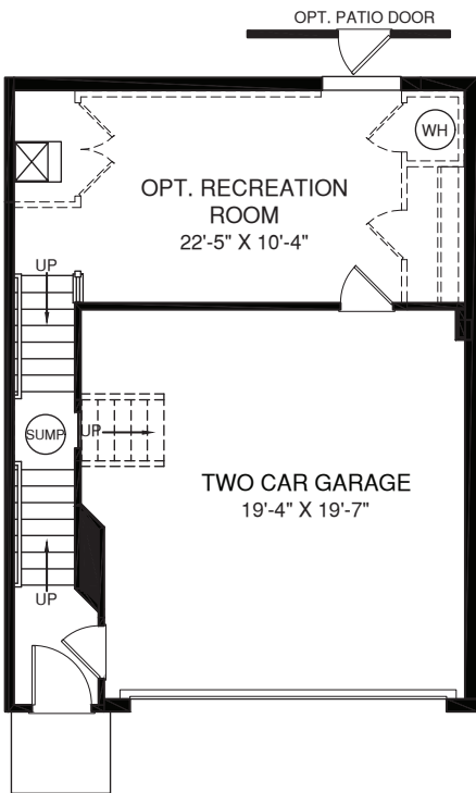
LOWER LEVEL
