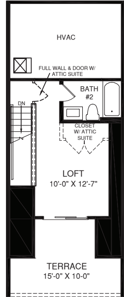
FOURTH FLOOR
