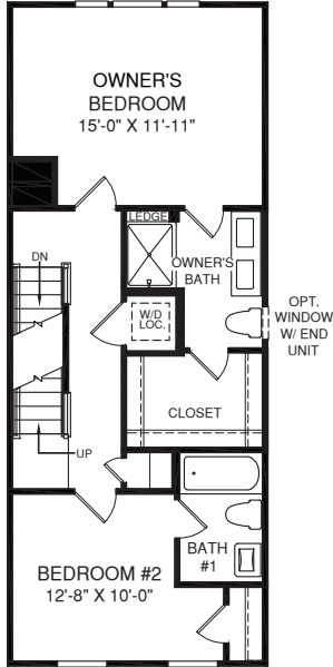
THIRD FLOOR
