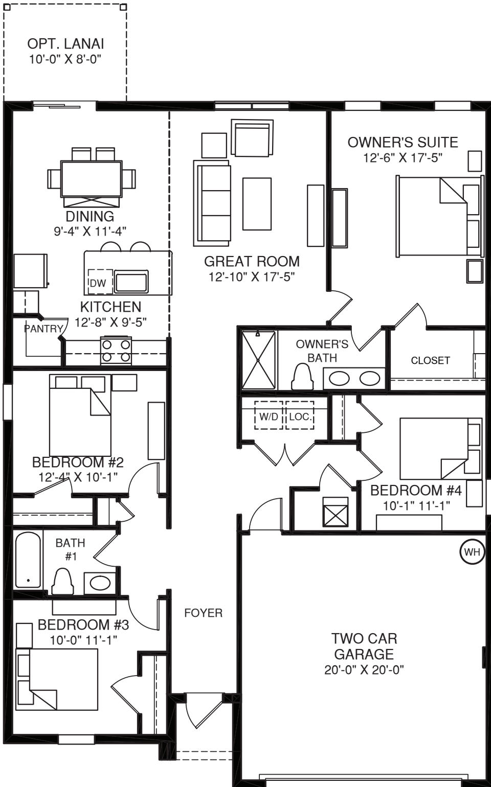
MAIN LEVEL
