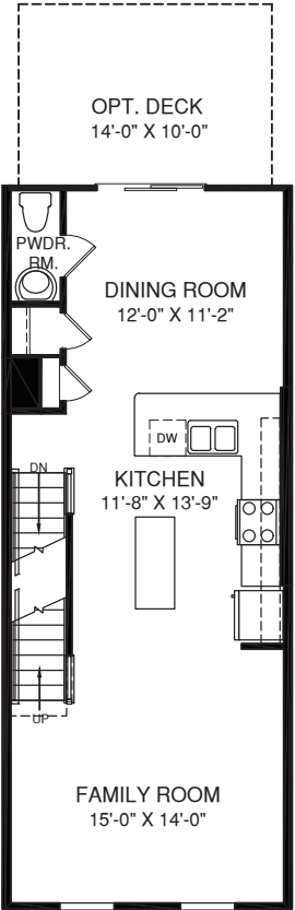
SECOND FLOOR
