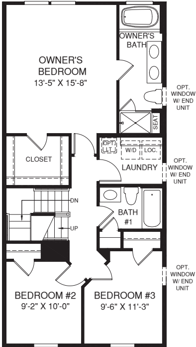
UPPER & ATTIC LEVEL
