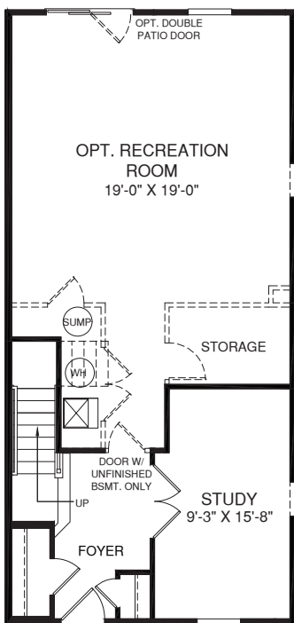
LOWER LEVEL
