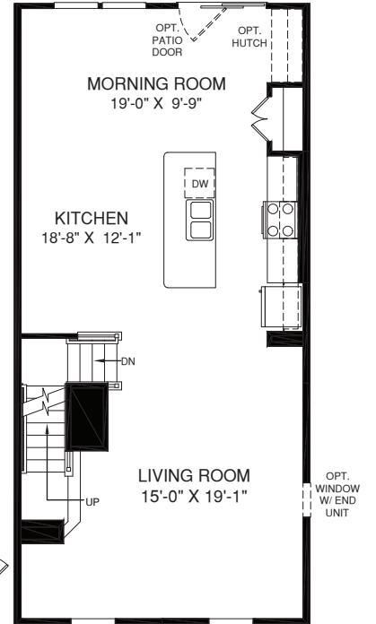
MAIN LEVEL
