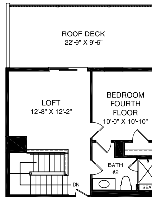
OPT. BEDROOM FOURTH FLOOR W OPT. 4'-0" EXTENSION TO HOUSE
