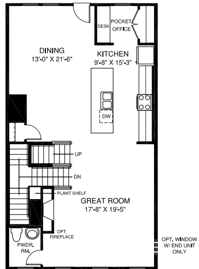
OPT. 4'-0" EXTENSION TO HOUSE
