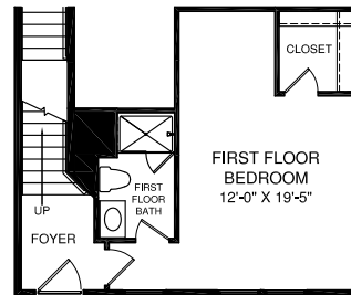
OPT. FIRST FLOOR BEDROOM W/ OPT. 4'-0" EXTENSION TO HOUSE
