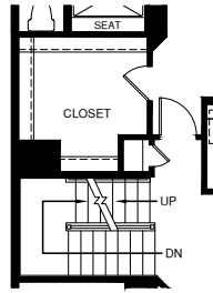
STAIRS W/ OPT. FOURTH FLOOR BEDRM. AND 4'-0" EXTENSION TO HOUSE
