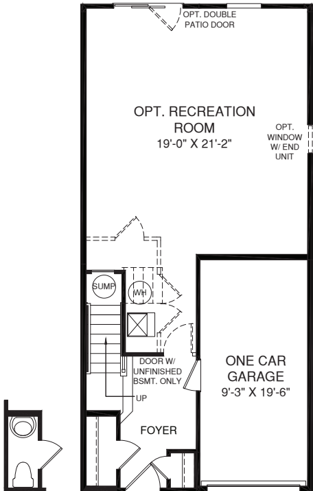
LOWER LEVEL
