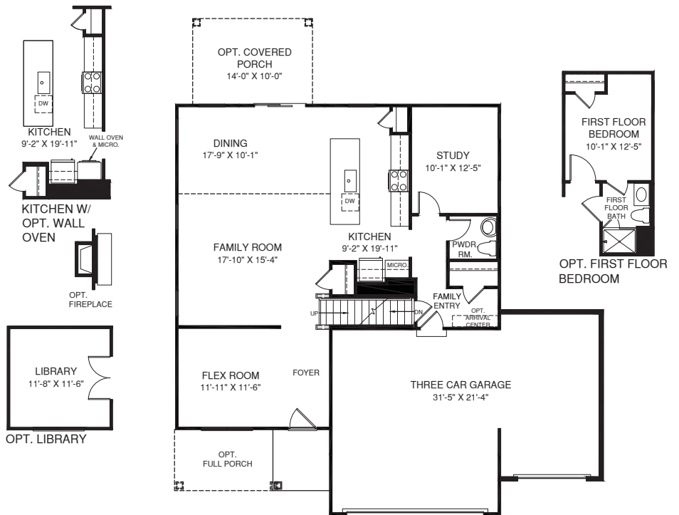
MAIN LEVEL
