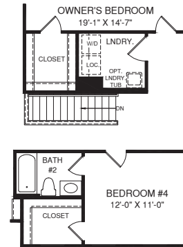
OPT. BATH #2
