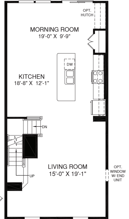
MAIN LEVEL
