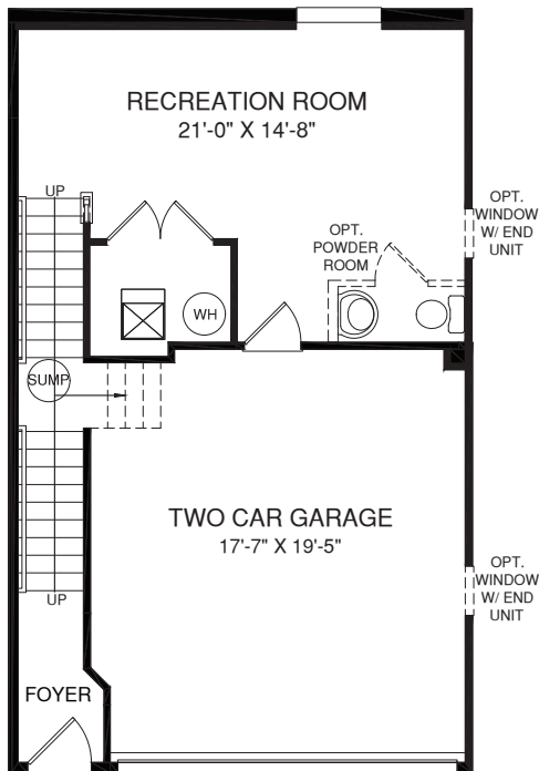
LOWER LEVEL
