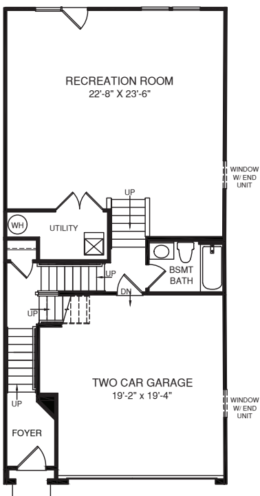
LOWER LEVEL
