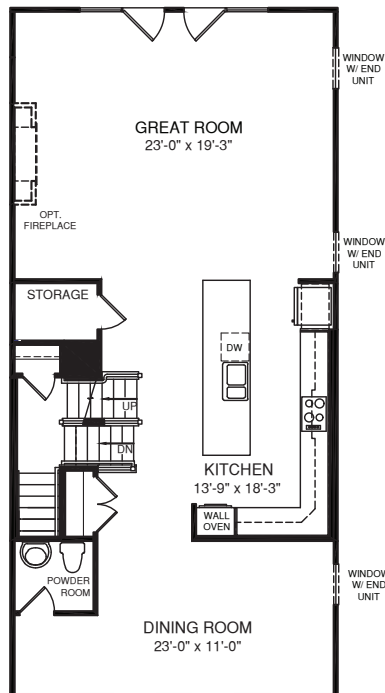
MAIN LEVEL
