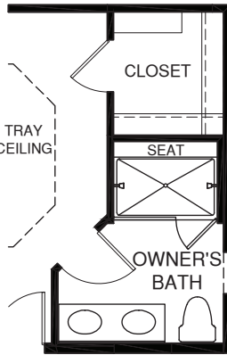
OPT. OWNER'S BATH SHOWER ALT. LAYOUT
