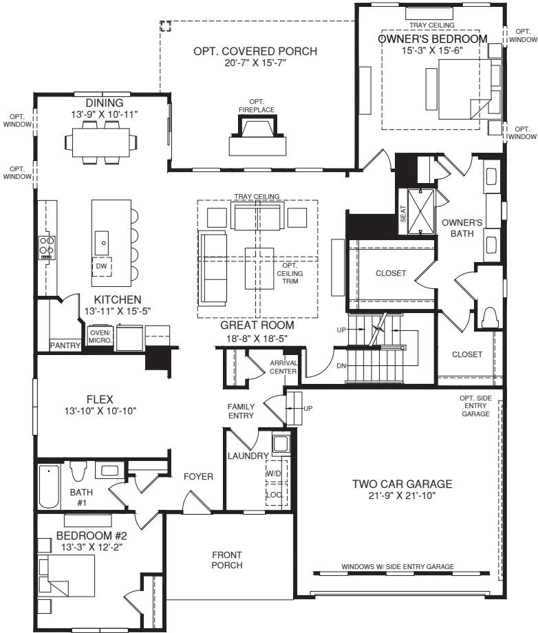
OPT. KITCHEN CABINET HOOD SHOWN W/ OPT. BEDROOM FIRST FLOOR
