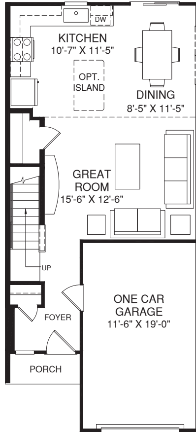
MAIN LEVEL
