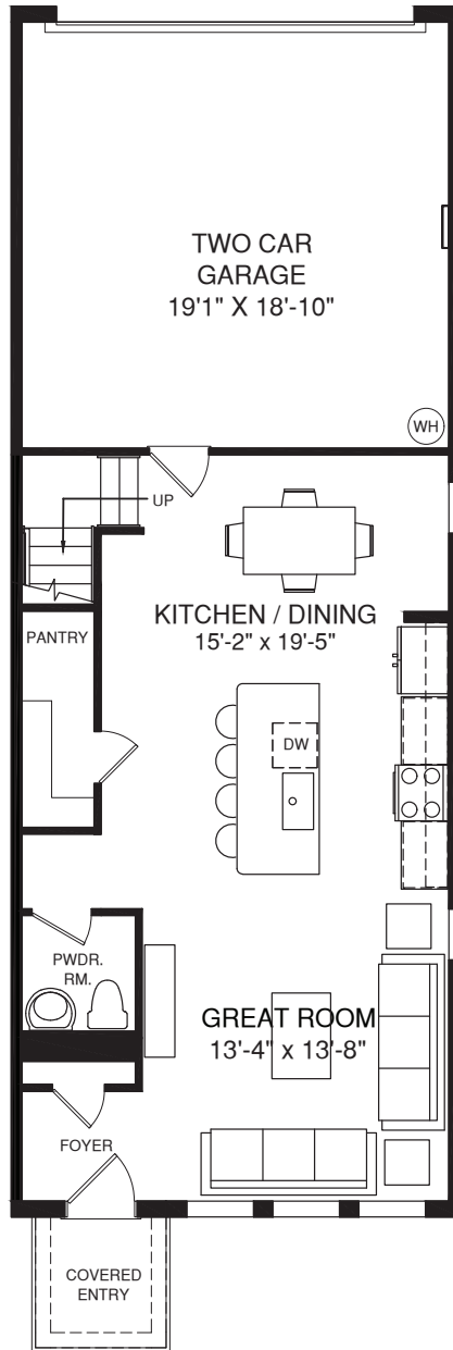
MAIN LEVEL
