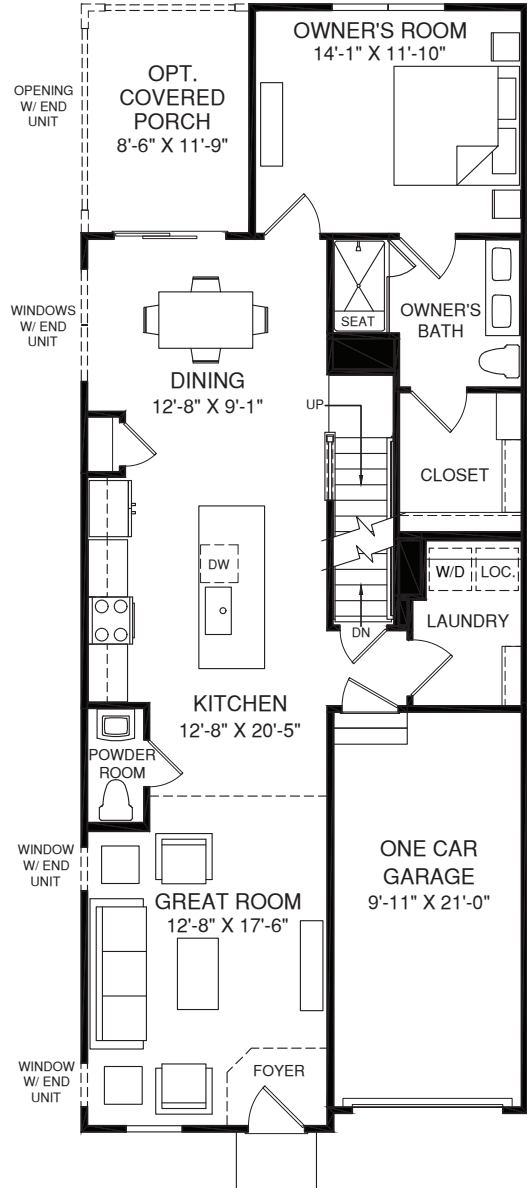
MAIN LEVEL
